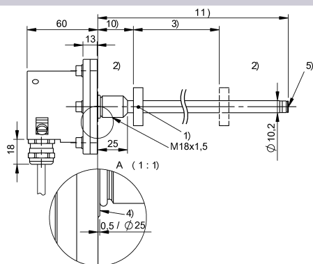
BTL5-Sxxxx-Mxxxx-B-DEXB-Kxx
