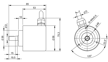
Cable outlet radial
