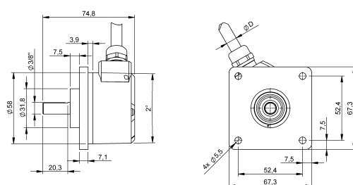
Cable outlet radial
