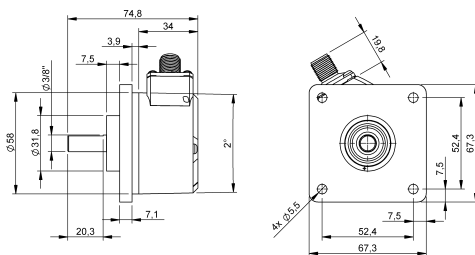
Connector outlet radial
