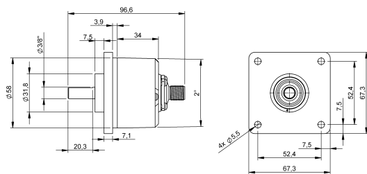
Connector outlet axial
