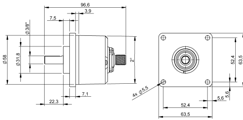
Connector outlet axial
