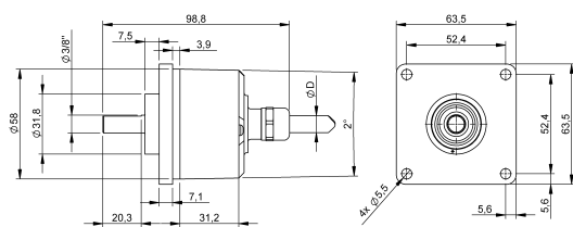
Cable outlet axial
