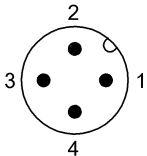
M12x1-male, 4-pin, A-coded
