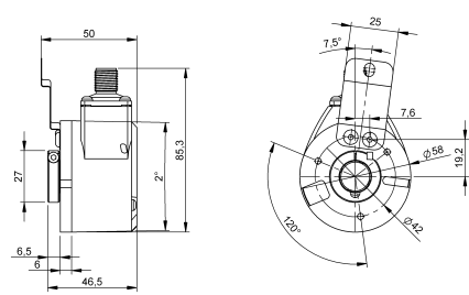
Connector outlet radial (optical)
