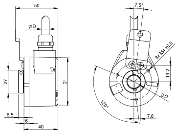
Cable outlet radial (optical)
