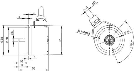
Cable outlet radial
