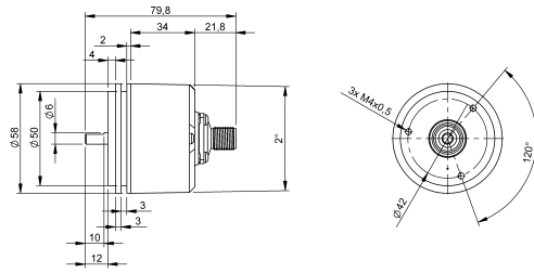
Connector outlet axial
