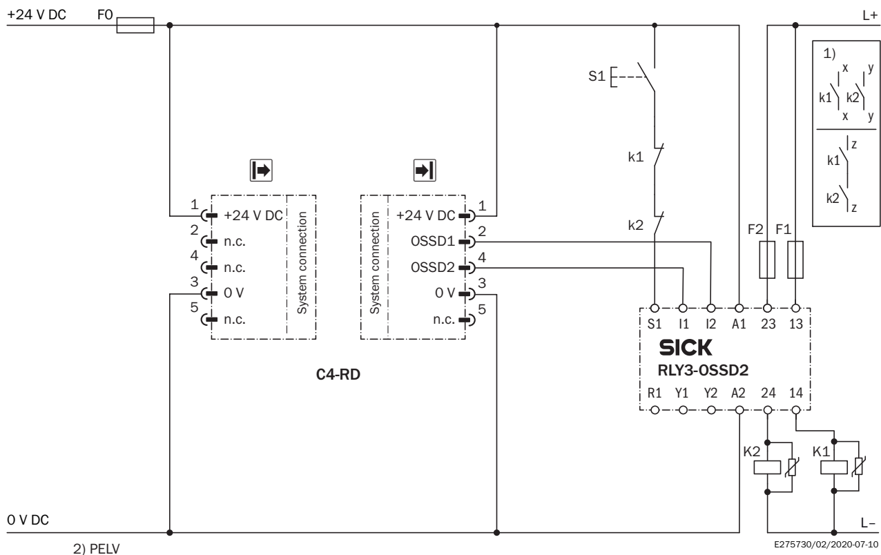
Connection diagram C4-RD safety light curtain on RLY3-OSSD200 safety relay
